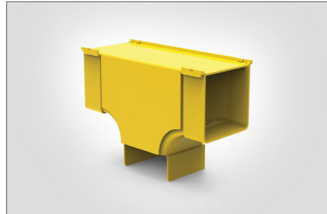
100x100mm Vertical T-Junction.
