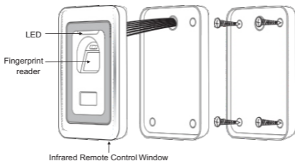
Installation drawing
